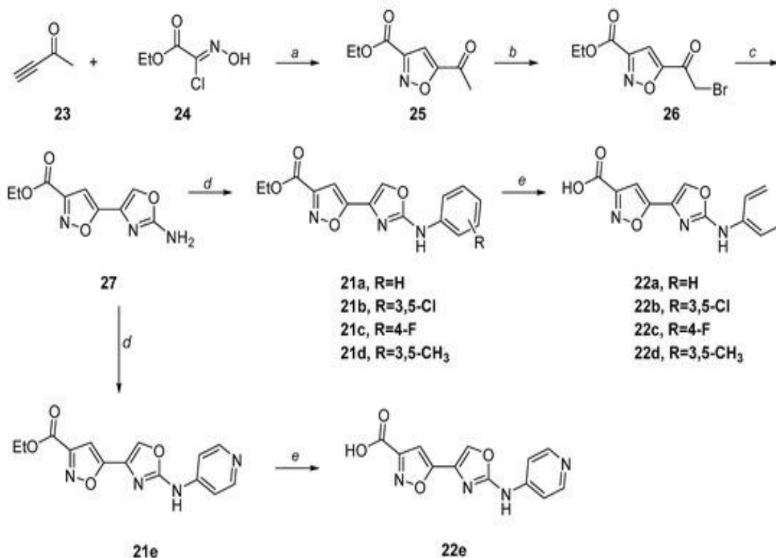
Scheme 1. a Reagents and conditions: (a) triethylamine, tetrahydrofuran, room temperature (b) N-bromosuccinimide, p -toluenesulfonic acid, acetonitrile, reflux (c) urea, dimethylformamide, microwave
