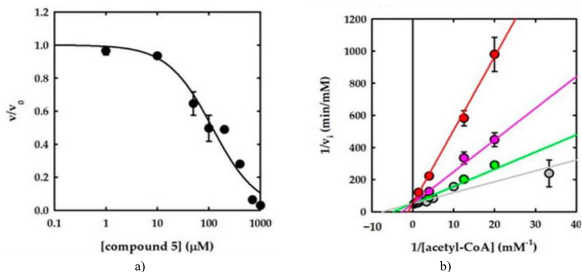
Figure 3. Inhibition profile of compound 5. (a) Relative initial reaction velocity as a function of compound 5 concentration. Experimental data were fitted to Equation 1, yielding an IC_{50} value of 110 \pm 0 \mu\text{M} . (b) Initial reaction rates measured at increasing acetyl-CoA concentrations in the absence of inhibitor (grey symbols) and in the presence of compound 5 at 30 \mu\text{M} (green symbols), 100 \mu\text{M} (pink symbols), and 300 \mu\text{M} (red symbols). Data were fitted using the linearized form of Equation 2, providing a K_i value of 64 \pm 12 \mu\text{M} .
