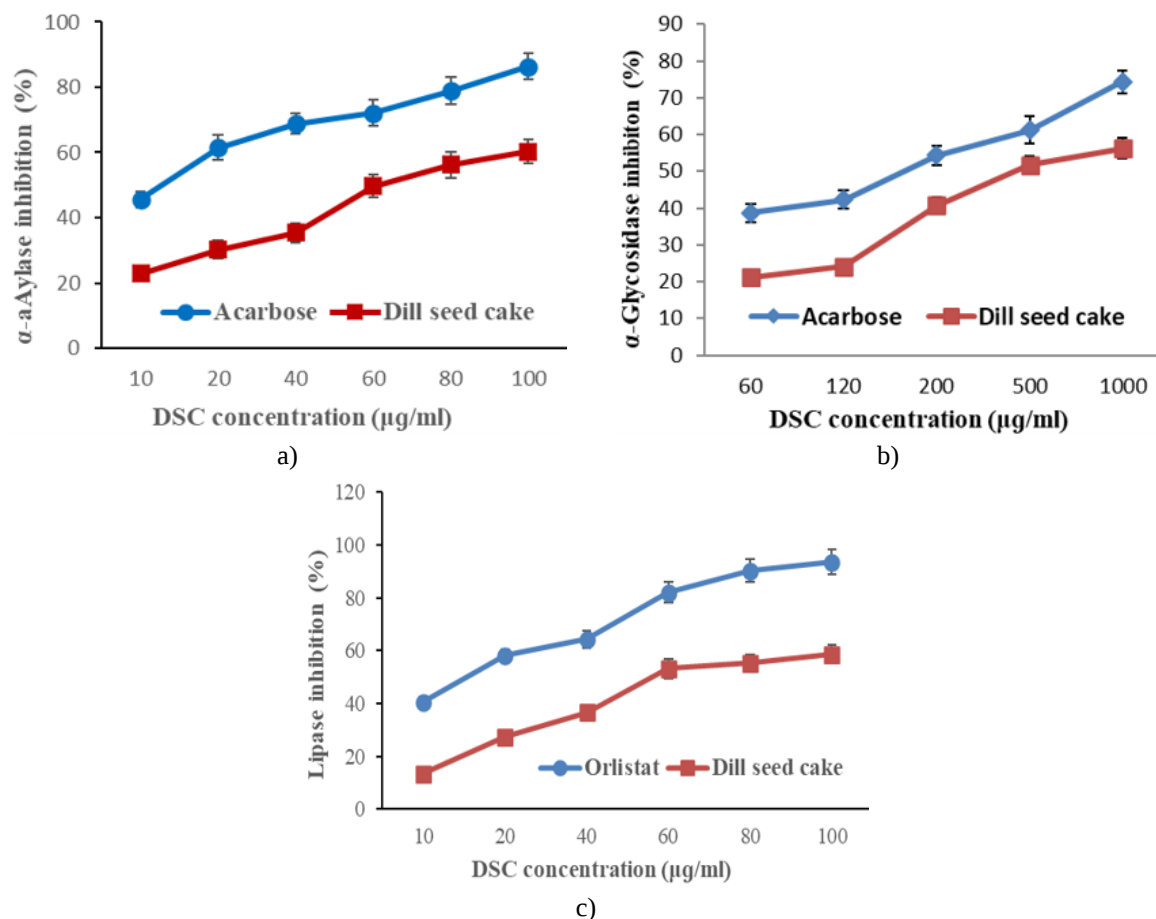
Figure 4. \alpha -Amylase, \alpha -glycosidase, and lipase inhibitory activity of dill seed cake at different concentration ranges.
