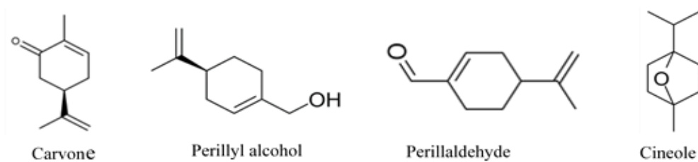
Figure 1. Chemical structure of dill seed lignan
