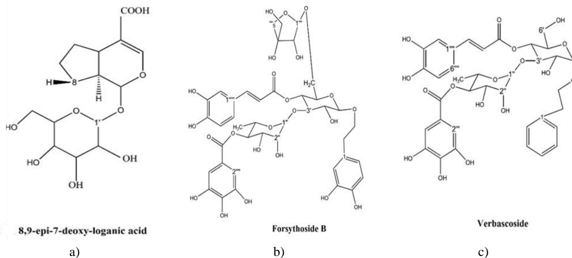
Figure 1. Chemical structures of compounds isolated from Nepeta racemosa .
