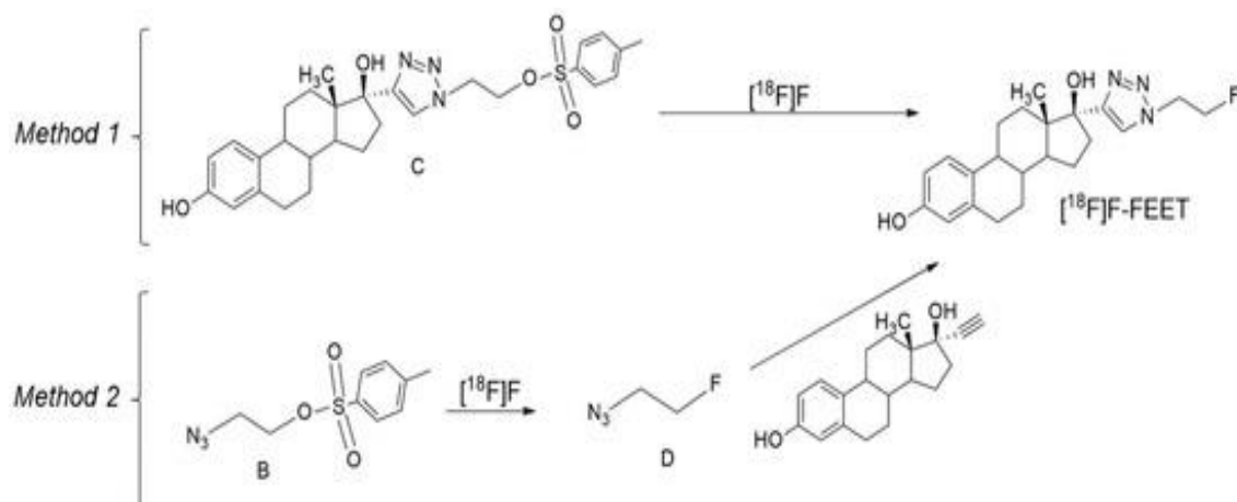
Figure 3. Synthesis of [^{18}\text{F}]\text{F-FEET} by methods 1 and 2.
