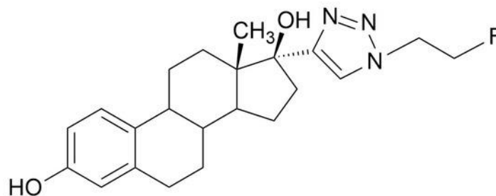
Figure 2. Structure of [^{18}\text{F}]\text{F-FEET} .
