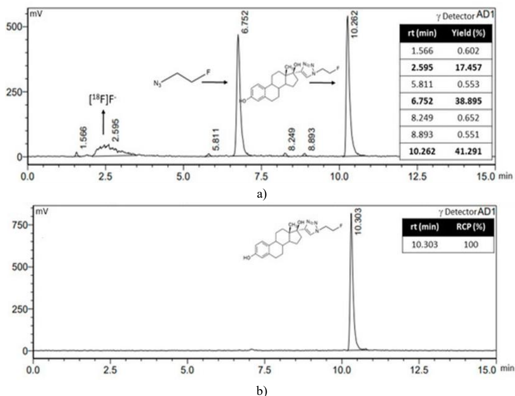
Figure 7. (a) Chromatographic profile obtained for entry 9 of Table 2 ; (b) Chromatographic profile obtained after the purification of ^{18}\text{F} -FEET.
