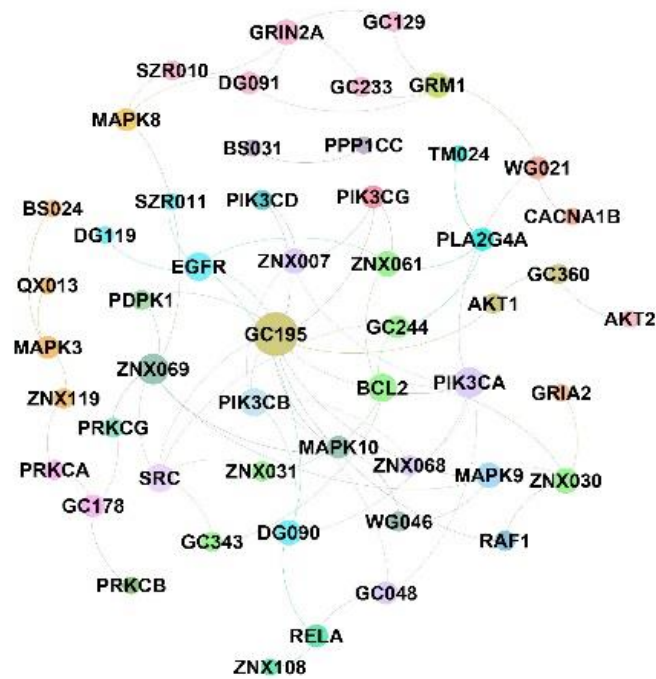
Figure 2. Network analysis: a) the key pathway-target network, and b) the core target-compound network.
