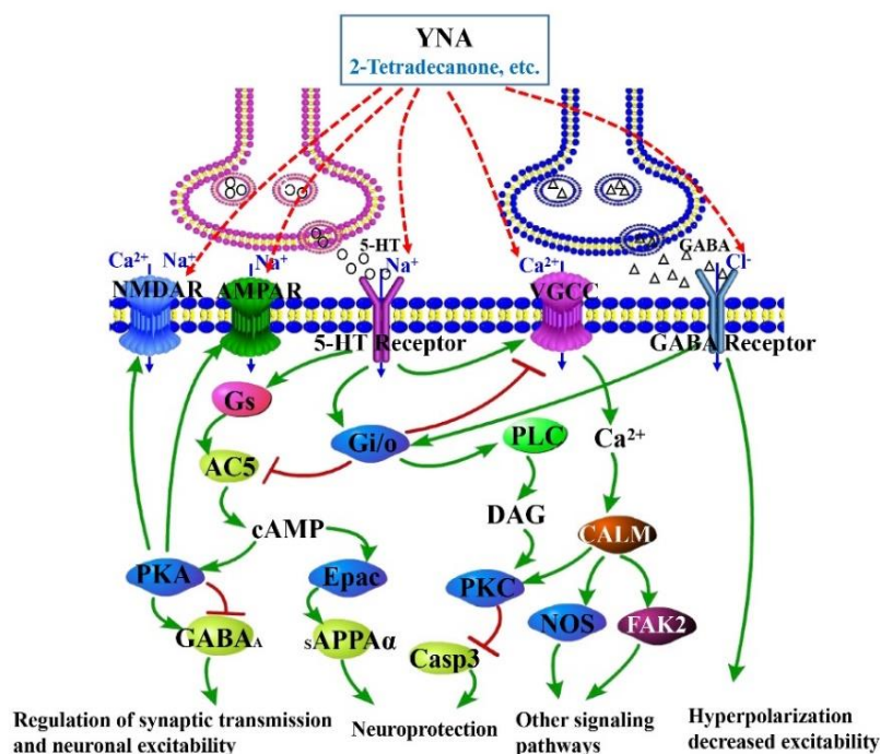
Figure 4. The potential mechanism of YNA in treating epilepsy.
