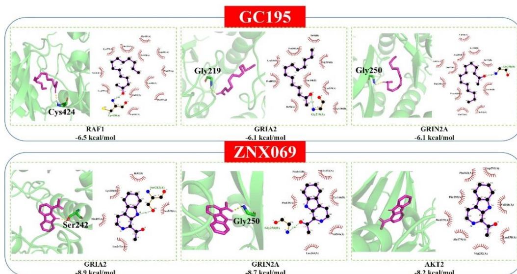
Figure 3. The predicted binding mode of GC195 and ZNX069 to their respective top three-scoring targets.
