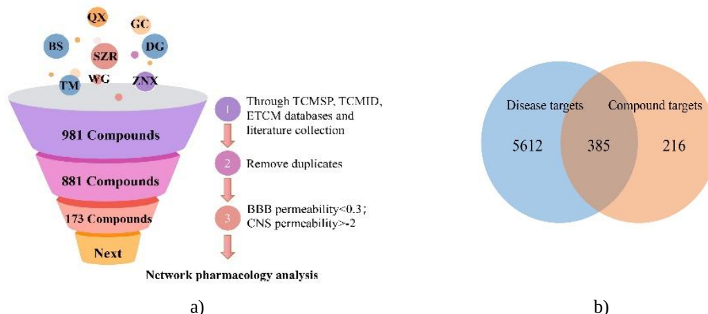
Figure 1. a) The compounds screening process, and b) Venn map of YNA target for treating epilepsy.
