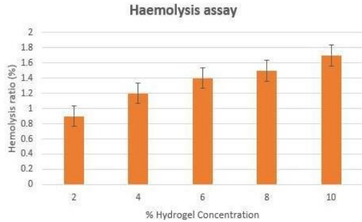
Figure 1. Hemolysis assay
