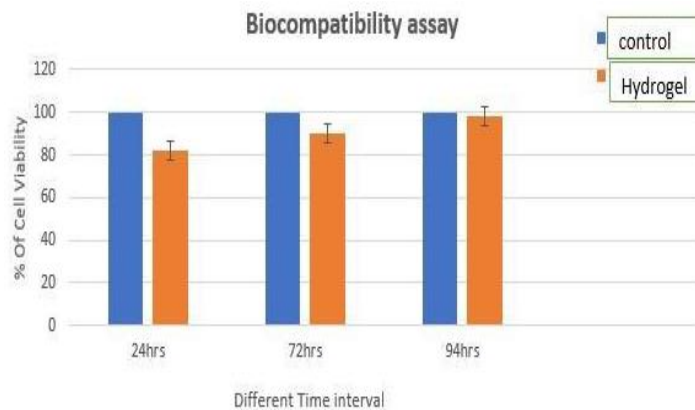
Figure 2. Biocompatibility assay
