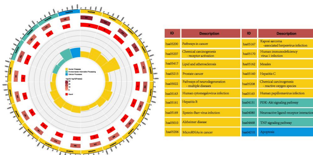
Figure 5. KEGG pathway enrichment analysis.
