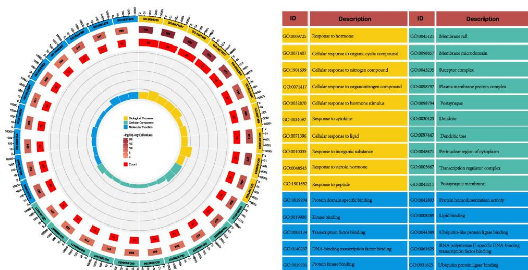
Figure 4. GO term enrichment analysis.
