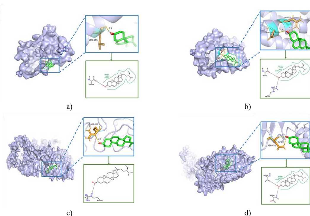
Figure 7. Visualization of molecular docking results, shown in both 3D and 2D representations: (a) IL6– \beta -sitosterol; (b) IL6–stigmasterol; (c) ESR1– \beta -sitosterol; (d) ESR1– \beta -sitosterol.
