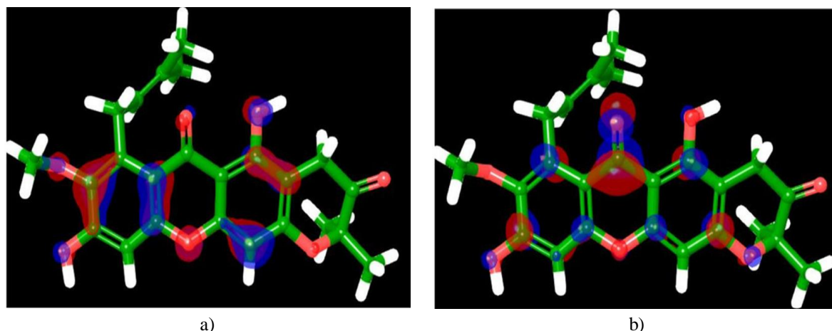
Figure 14. Spatial Distribution of HOMO (A) and LUMO (B) orbitals in hit 8.
