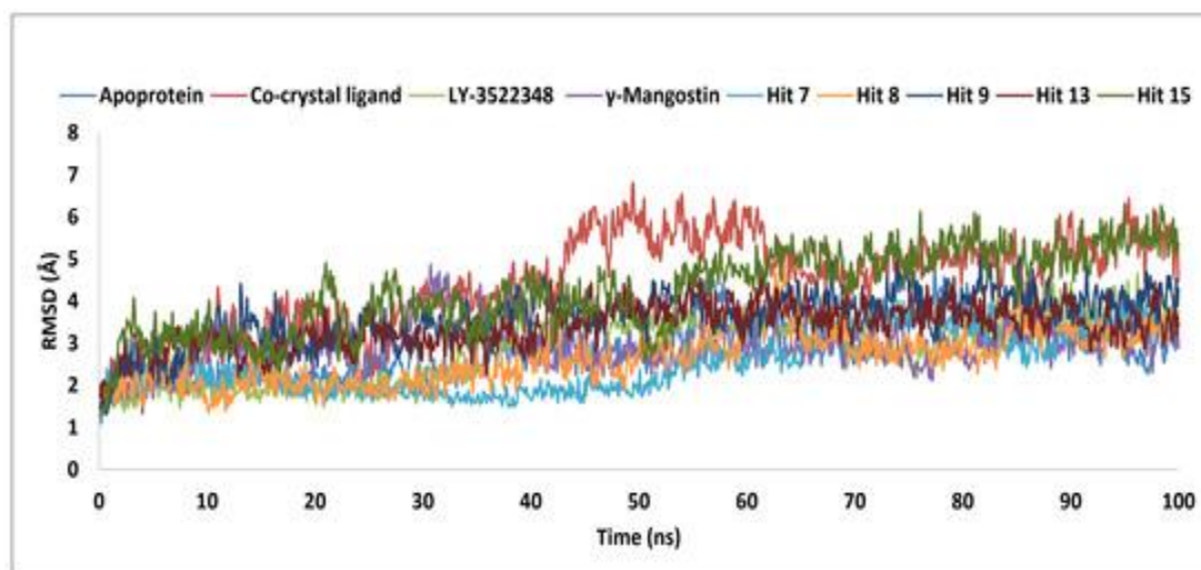
Figure 11. Root mean square deviation (RMSD) evaluation of compounds 7, 8, 9, 13, 15, \gamma -Mangostin, LY-3522348, the co-crystallized ligand, and the unbound protein throughout 100 ns molecular dynamics simulations.
