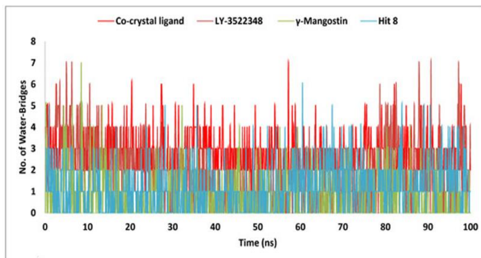
Figure 13. Evaluation of hydrogen bonds (a), hydrophobic interactions (b), and water-mediated bridges (c) for the co-crystallized ligand, LY-3522348, \gamma -Mangostin, and hit 8 across 100 ns molecular dynamics simulations.
