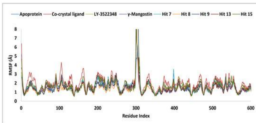
Figure 12. Root mean square fluctuation (RMSF) evaluation of compounds 7, 8, 9, 13, 15, \gamma -Mangostin, LY-3522348, the co-crystallized ligand, and the ligand-free protein, illustrating amino acid residue flexibility across 100 ns molecular dynamics simulations.
