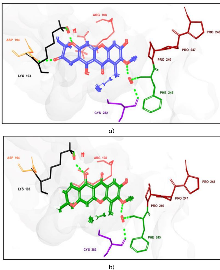
Figure 7. 3D binding modes of two prenylated xanthenes, designated as hit 8 (panel a) and hit 13 (panel b), within the active site of KHK-C (PDB ID: 8UG1). These visualizations emphasize critical amino acid contacts, including hydrogen bonds and water-mediated bridges (shown in green) as well as \pi -cation interactions (depicted in red).
