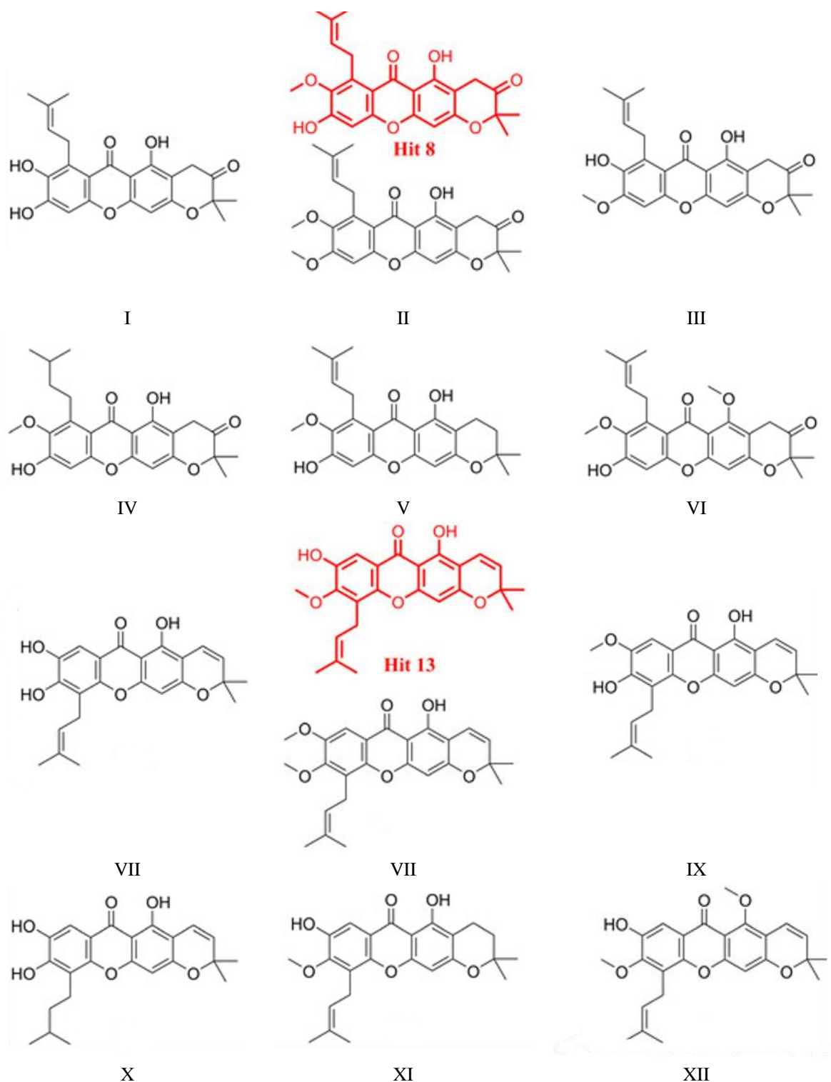
Figure 8. Structures of the proposed analogs based on hit 8 (labeled I–VI) and hit 13 (labeled VII–XII).
