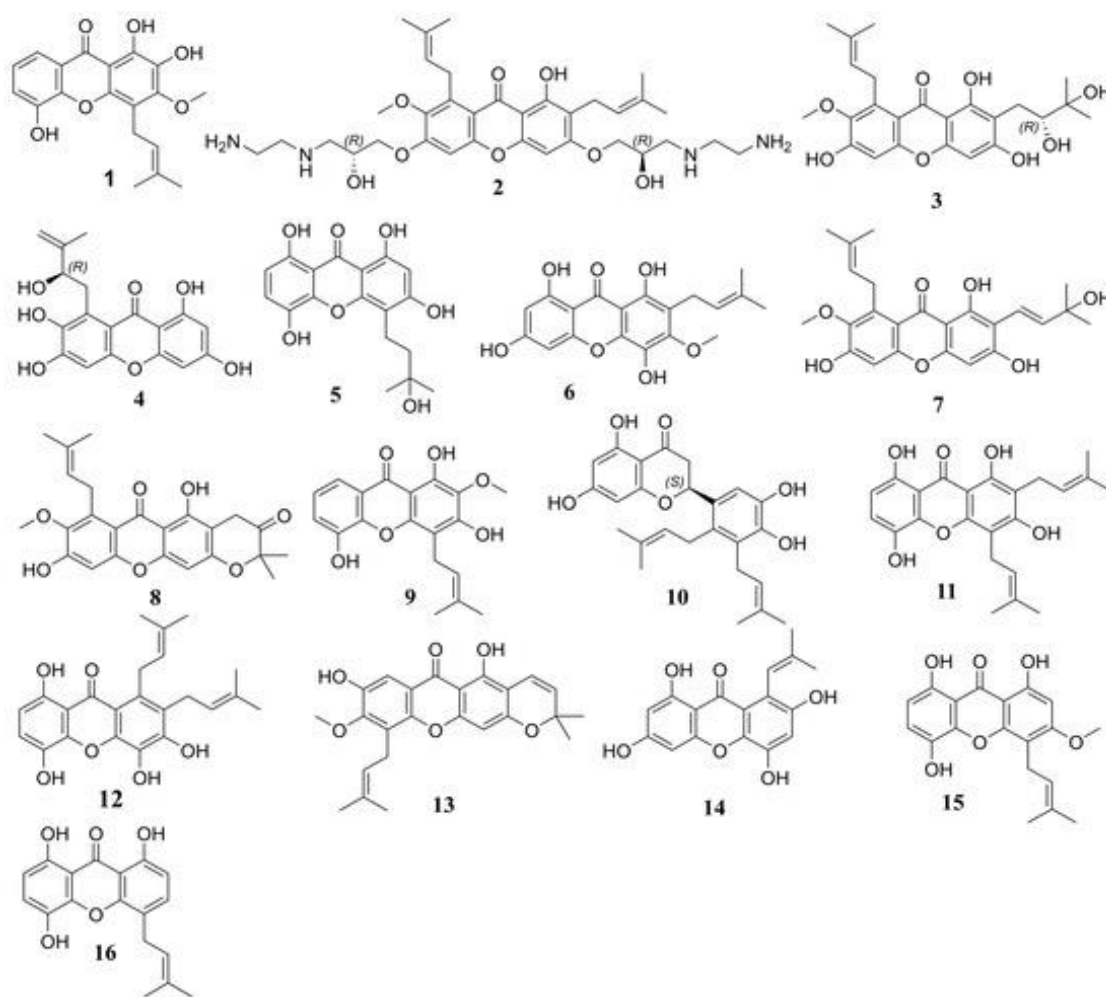
Figure 6. Structural representations of the primary hit compounds obtained from the virtual screening workflow.
