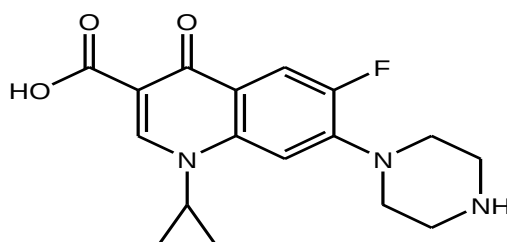
Figure 1. Ciprofloxacin
