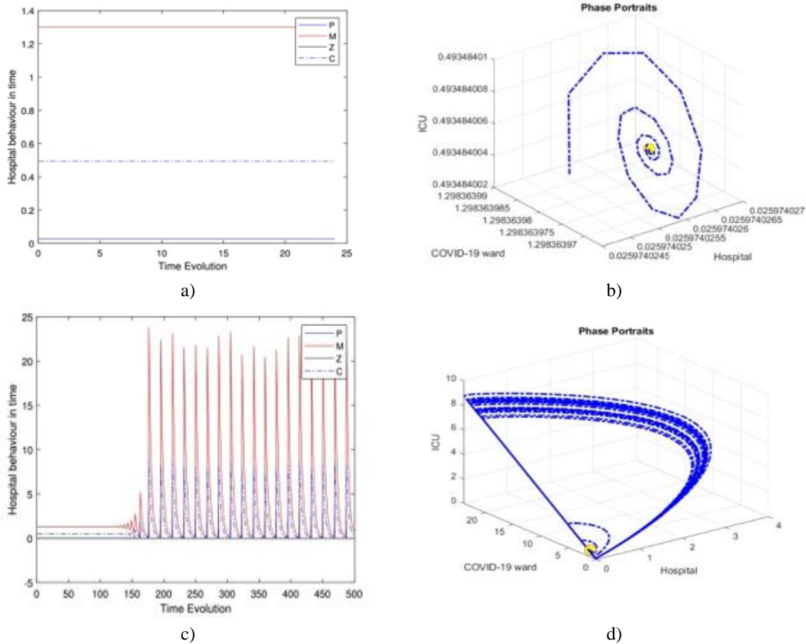
Figure 6. Time series and phase-space trajectories near the proposed initial condition for the third positive root of the quartic polynomial, representing the clinically relevant equilibrium E_4 over 24-hour and 500-hour intervals. Eq. (13) defines this equilibrium, and all other parameters remain as in Table 2 .
