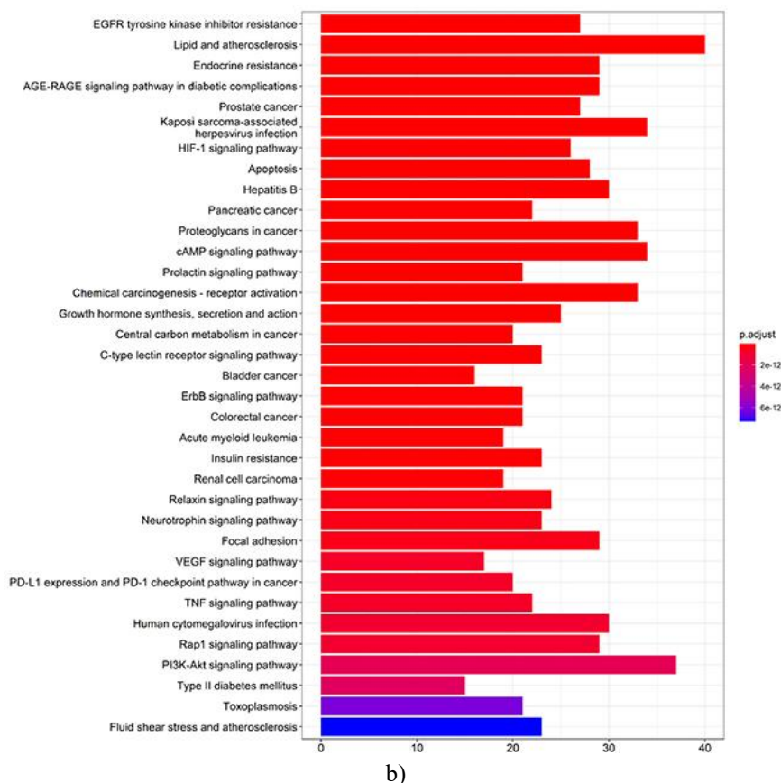
Figure 5. GO enrichment and KEGG pathway analysis identified critical pathways associated with ZGJTSXF. (a) The top 10 enrichment items of Biological Process, Molecular Function and Cellular Components from GO enrichment analysis. (b) The top 35 pathways of KEGG pathway analysis.
