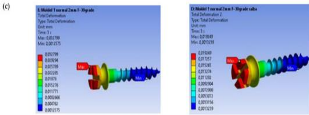
Figure 4. Comparative evaluation of (a) von Mises stresses, (b) linear deformations, and (c) total displacements for implants with and without SD
