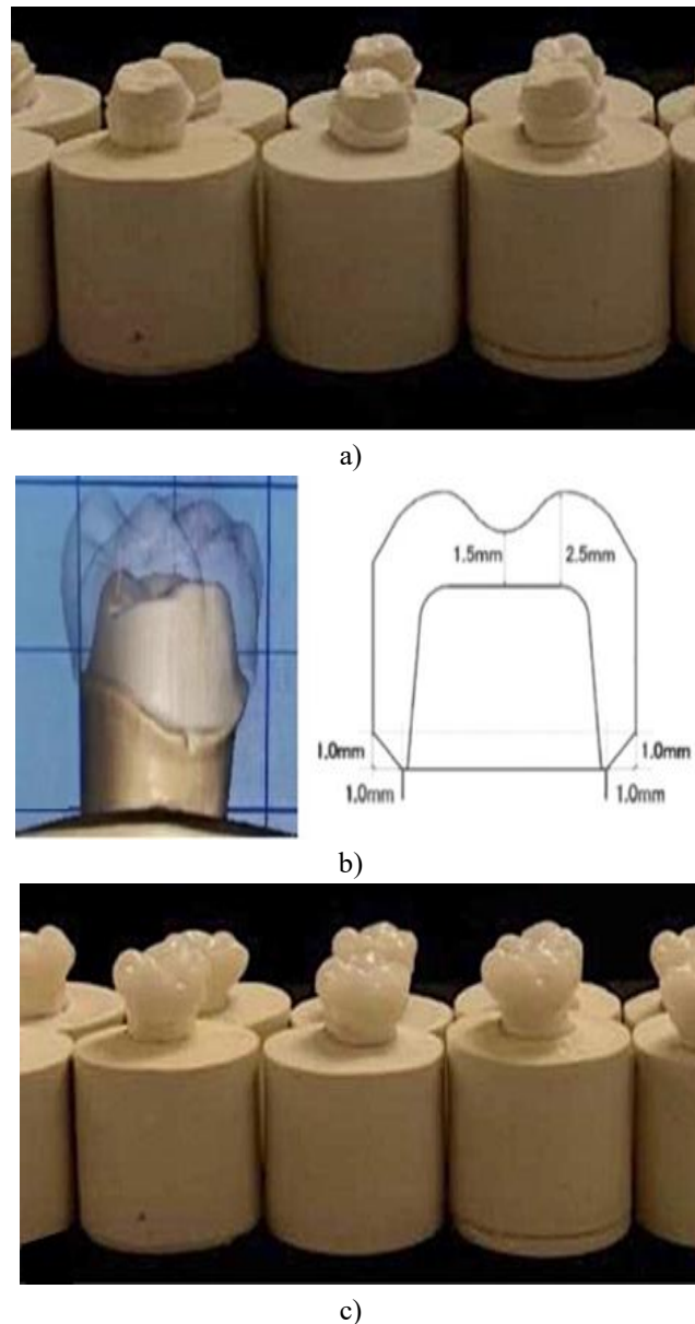
Figure 3. Resin test blocks; a) resin test blocks with embedded duplicate abutment teeth, b) digital scan and design of the tested PICN hybrid ceramic crown, and c) resin test blocks with cemented crowns.
